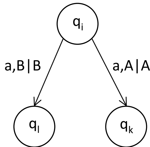
DPDA
